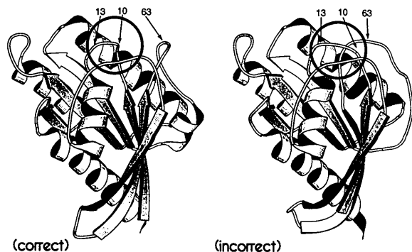
Fig. 2. Ribbon drawings of the correct and partially incorrect structures of p21. The dark circle is drawn around the region where the omit-map calculations were directed. Here, the \beta -strand crossover is apparent by the change in the conformation of the loops around residue 10 and residue 63. In the omit-map calculations, residues within 5 Å of residue 10 were removed from the incorrect structure.
