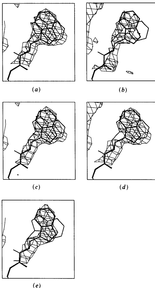
Fig. 6. The effects of various omit-map techniques around Trp 91 located in the light chain of the AN02 Fab fragment. The correct conformation of Trp 91 is shown in black, the initial incorrect conformation is shown in gray. All maps are of the \sigma_A -weighted 2F_o - F_c type (see Methods) at 2.8 Å resolution. Residues 89–97 in the light chain, 93–102 from the heavy chain, and the hapten molecule were omitted for all map calculations and refinements. (a) Ordinary omit map of the initial incorrect structure shown at a contour level of 1.2\sigma . (b) The fourth iteration of density modification on the initial incorrect structure shown at a contour level of 0.7\sigma . The region of modification was defined by a 2.0 Å cushion around the omitted region. (c) Minimized omit map of the initial structure shown at a contour level of 1.2\sigma . The partial structure was refined through 120 cycles of conjugate-gradient minimization at 8.0–2.8 Å resolution. (d) Randomized and minimized omit map of the initial structure shown at a contour level of 1.2\sigma . (e) SA omit map of the initial structure shown at a contour level of 1.2\sigma . The partial structure was refined using a SA slow-cooling protocol (Brünger et al. , 1990) with a starting temperature of 3000 K at 8.0–2.8 Å resolution.
