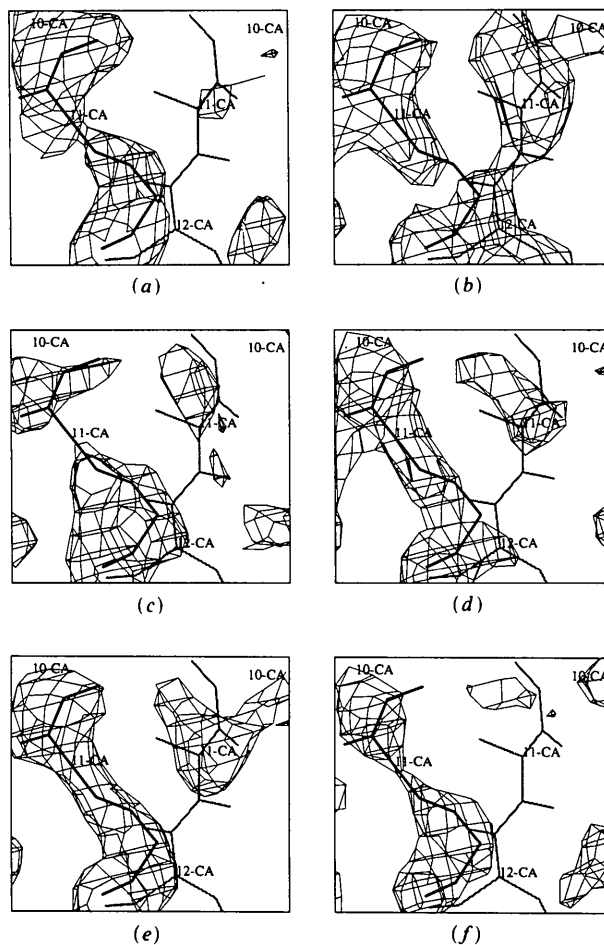
Fig. 3. The effects of various omit-map techniques around residues 10–12 in p21. The correct branch is shown in black, the incorrect branch is shown in gray. All maps are of the \sigma_A -weighted 2F_o - F_c type (see Methods ) at 2.25 Å resolution. (a) Ordinary omit map of the correct structure shown at a contour level of 1.2\sigma . (b) Ordinary omit map of the incorrect structure shown at a contour level of 1.2\sigma . All residues within 5 Å of residue 10 were omitted in all calculations. (c) Omit map after four iterations of density modification shown at a contour level of 0.6\sigma . The density-modification region was defined by a 2.0 Å cushion around the omitted atoms. (d) Minimized omit map of the incorrect structure shown at a contour level of 1.0\sigma . The partial structure was refined through 120 cycles of conjugate-gradient minimization at 8.0–2.25 Å resolution. (e) Randomized and minimized omit map of the partially incorrect structure shown at a contour level of 1.0\sigma . (f) SA omit map of the partially incorrect structure at 1.0\sigma . The partial structure was refined using the SA slow-cooling protocol (Brünger et al. , 1990) with a starting temperature of 3000 K at 8.0–2.25 Å resolution.
