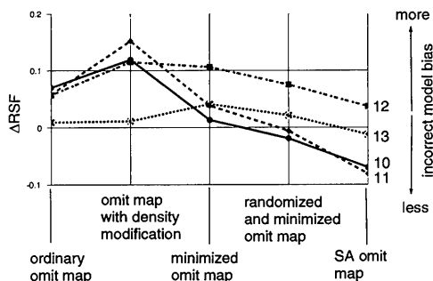
Fig. 4. The difference between the RSR calculated for the correct structure and that of the incorrect structure (Jones et al. , 1991). The RSR values for all backbone atoms of each residue of the incorrect branch site were subtracted from the values calculated for the corresponding residue in the correct structure. These values are plotted for the various \sigma_A -weighted 2F_o - F_c omit maps computed for the incorrect structure. The RSR is analogous to the R value used in crystallography. Thus, a small value signals a better fit. For the difference plotted here, a negative value denotes a better fit between the map and the correct structure than between the map and the same residue in the incorrect structure, i.e. less model bias towards the incorrect structure.
