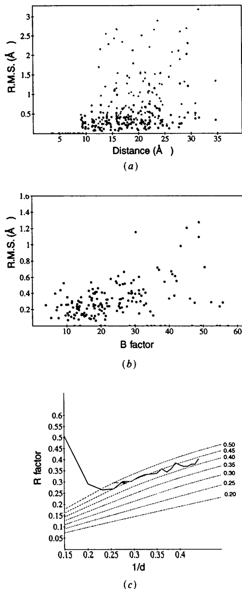
Fig. 5. The effects of the SA omit refinement on the coordinates of the incorrect model of p21. (a) Shown are the r.m.s. shifts in the coordinates of the backbone atoms (black dots) and side-chain atoms (gray dots) before and after the SA omit refinement of the residues of p21 versus the distance of that residue from residue 10 in the omitted region. (b) R.m.s. shifts in the coordinates of the backbone atoms before and after the SA omit refinement for each residue are plotted versus the average temperature factor of each residue's backbone atoms. (c) A Luzatti (1952) plot of the p21 data using the correct structure at 2.25 Å resolution.
