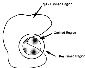
Fig. 1. A schematic representation of the simulated-annealing omit-map procedure. As described in Methods , the region in question is omitted from the structure. The atoms in a boundary region surrounding the omission are restrained to their starting coordinates. This restrained partial structure is then refined through simulated annealing to reduce the phase bias from the omitted region.
